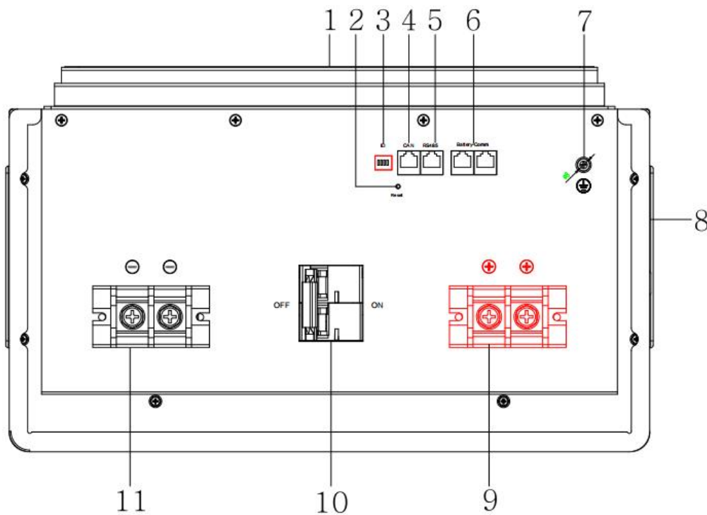
Figure 6-2 Front panel diagram(For both 25.6V &51.2V battery)
