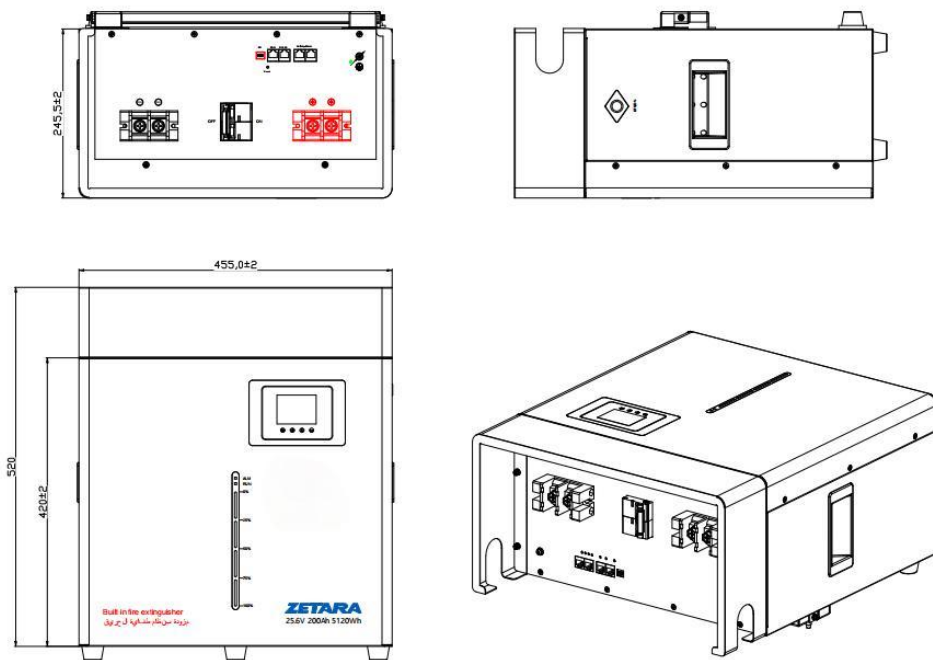
Figure 6-1-4 25.6V200Ah Appearance & dimension drawing
