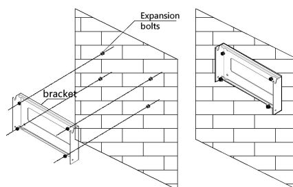
Figure 8-3 Bracket fixing
