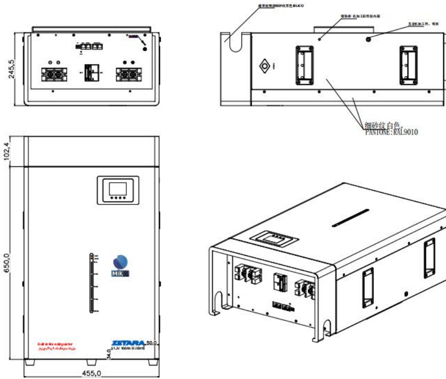
Figure 6-1-2 51.2V200Ah Appearance & dimension drawing
