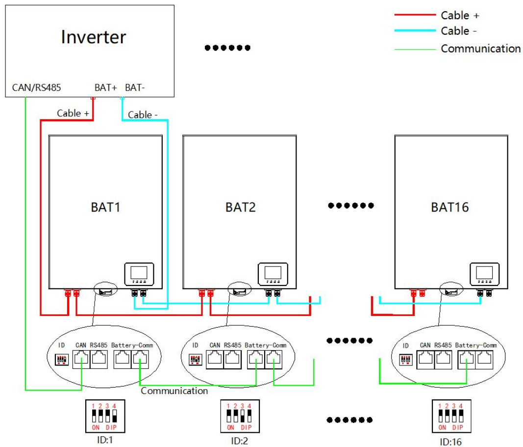
Figure 8-6 Multiple batteries in parallel schematic diagram
