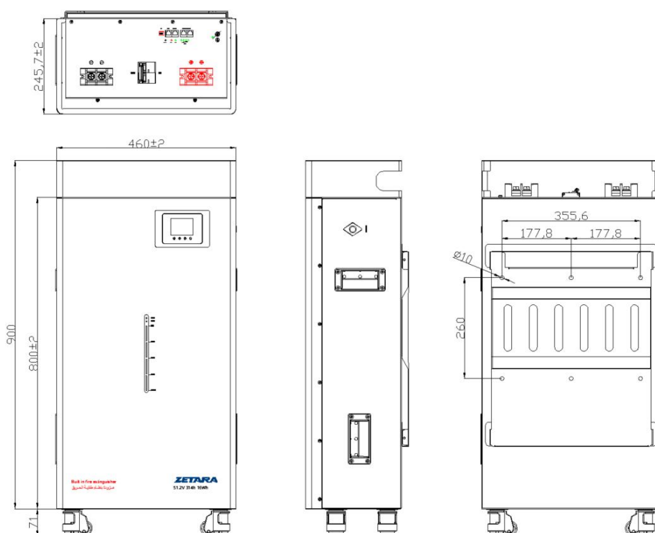
Figure 6-1-1 51.2V314Ah Appearance & Dimension drawing
