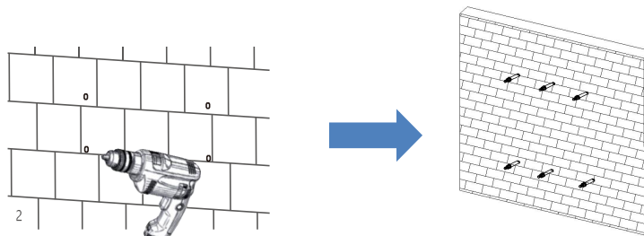
Figure 8-2 Expansion screws fixing
