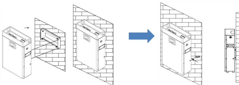
Figure 8-4 Install the battery bracket on the wall
