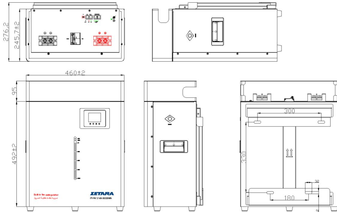
Figure 6-1-3 25.6V314Ah Appearance & dimension drawing
