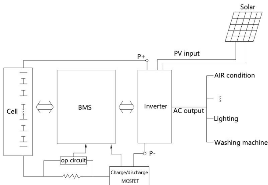
Figure 5-1 Working principle diagram of battery system
